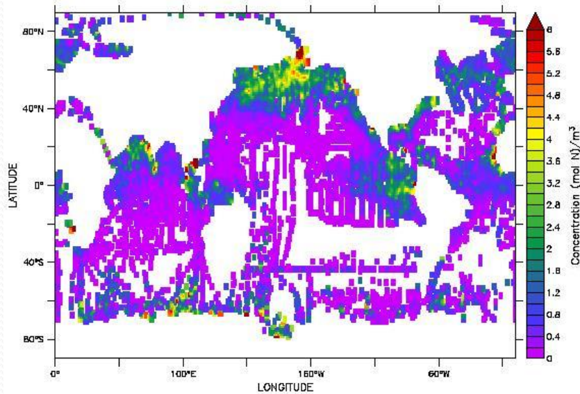
Mesozooplankton Observation
