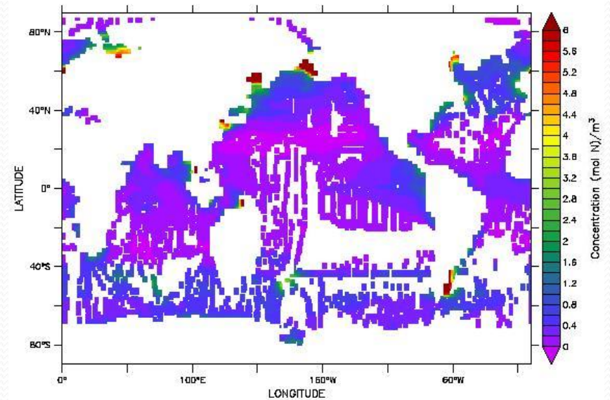
Mesozooplankton Model
